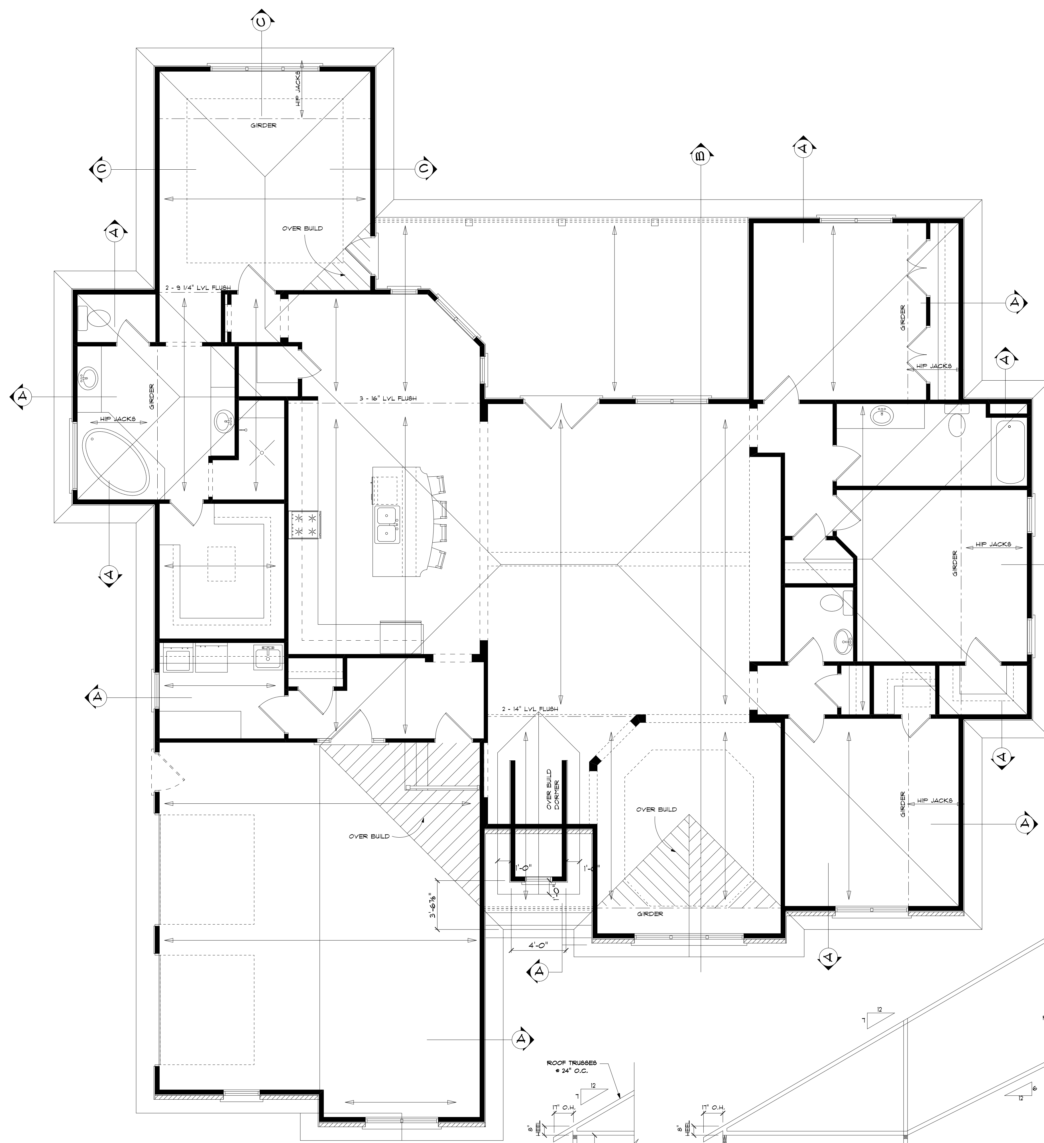
ROOF PLAN SCALE: 1/4"=1'-0"
